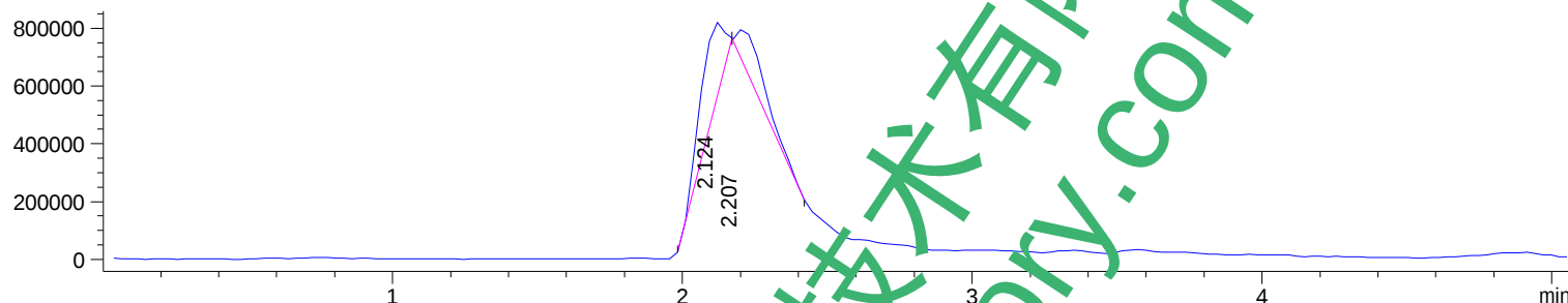
MSD2 TIC, MS File ES-API, Neg, Scan, Frag: 70 *** NO MS PEAKS INTEGRATED ***
